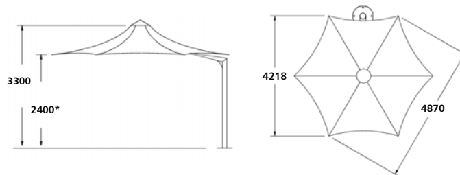
FLEXSHADE *16 HEXAGONAL
