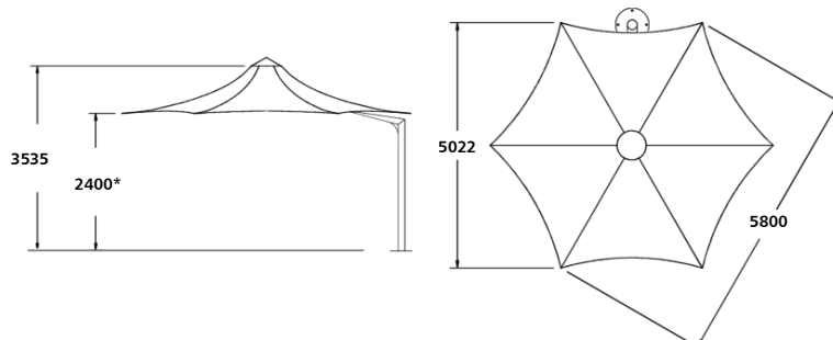
FLEXSHADE *19 HEXAGONAL
